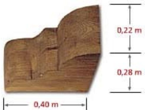
Wood Corbel CO B
